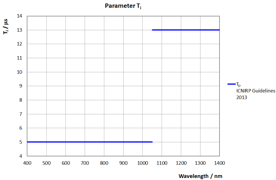
Figure A12: Parameter T_1 as a function of wavelength according to the ICNIRP guidelines on laser radiation [5].
