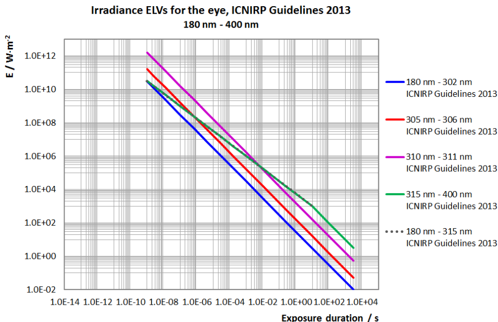
Figure A1: Irradiance ELVs for the eye of the ICNIRP guidelines on laser radiation [5] in the UV wavelength range between 180 nm and 400 nm. For exposure durations from 1 ns to 10 s, ELVs between 180 nm and 315 nm should not be exceeded (dotted line).
