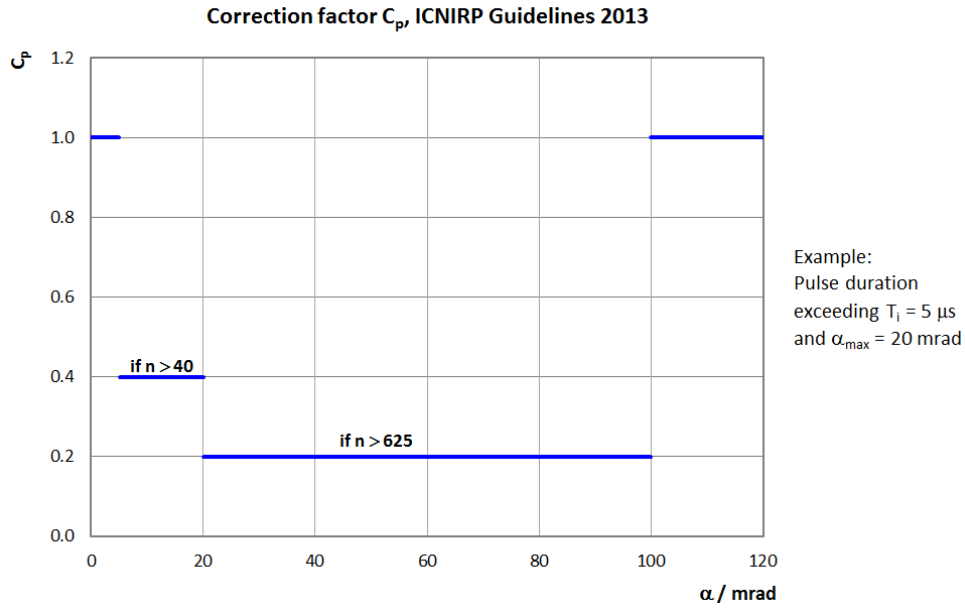
Figure A9: Correction factor C_p as a function of the angular subtense \alpha of a laser source according to the ICNIRP guidelines on laser radiation [5] for a pulse duration exceeding T_1 = 5 \mu\text{s} and \alpha_{\text{max}} = 20 \text{ mrad} ( t = 0.01 \text{ s} ). The factor accounts for the additivity of multiple pulses for thermally induced injury.
