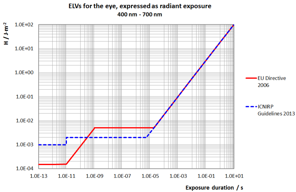
Figure A16: ELVs for the eye, expressed as radiant exposure, of the ICNIRP guidelines on laser radiation [5] and the Directive 2006/25/EC [1] in the visible wavelength range (between 400 nm and 700 nm).
