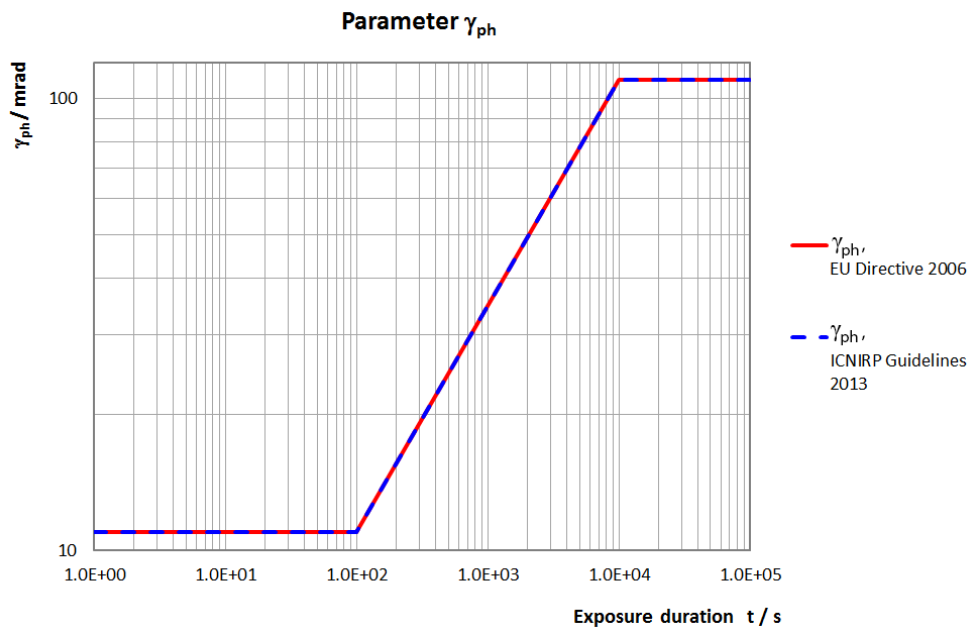
Figure A14: Parameter \gamma_{ph} , as a function of exposure duration, of the ICNIRP guidelines on laser radiation [5] and the Directive 2006/25/EC [1]. \gamma_{ph} is the measurement field of view (angle of acceptance).
